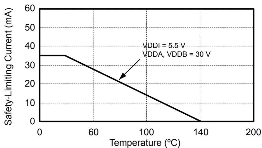
Figure 4.5. NB SOIC-8 Thermal Derating Curve, Dependence of Safety Limiting Values Limiting Values per VDE
