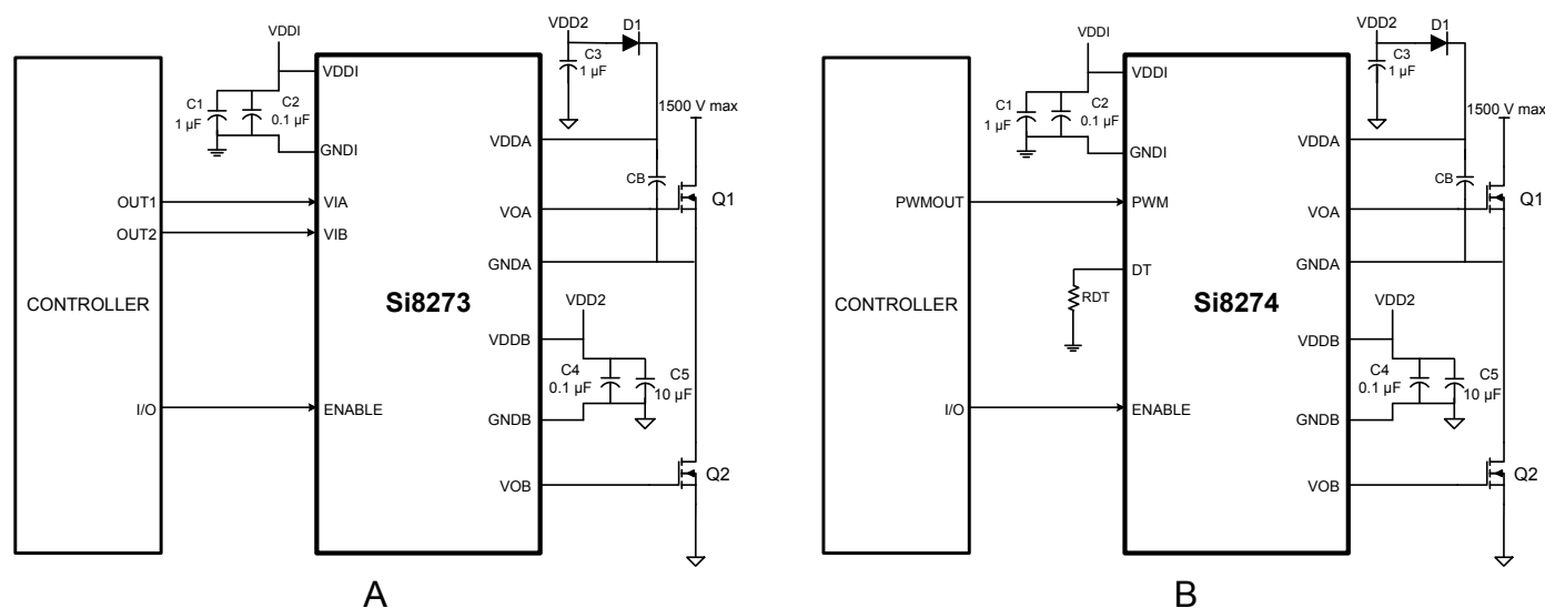
Figure 3.1. Si827x in Half-Bridge Application
