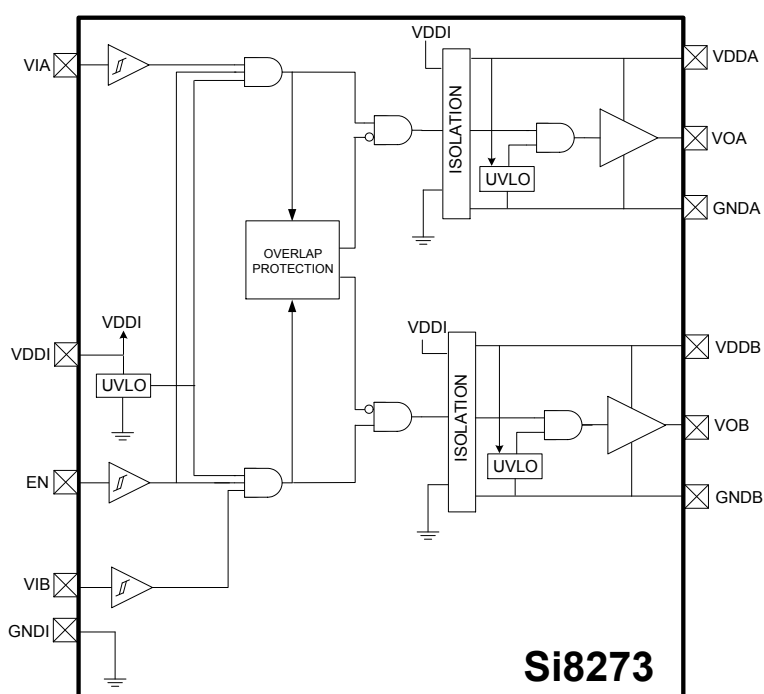
Figure 2.2. Si8273 Block Diagram
