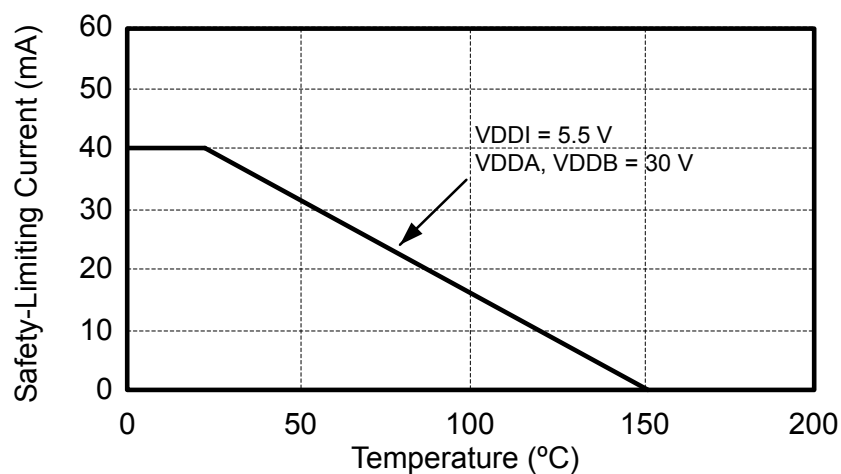
Figure 4.4. NB SOIC-16, QFN-14 Thermal Derating Curve, Dependence of Safety Limiting Values Limiting Values per VDE
